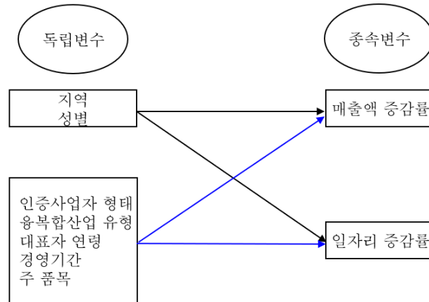
Figure 1. Research Model
