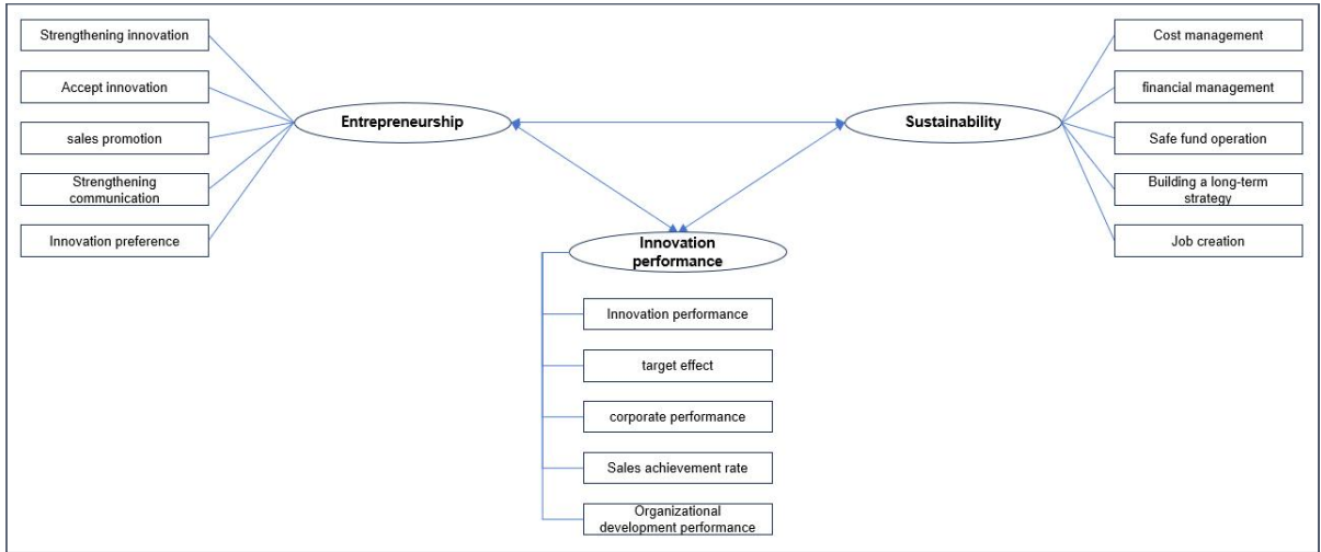
Figure 4. Research model
